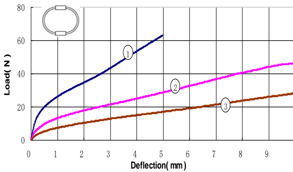
Compression
