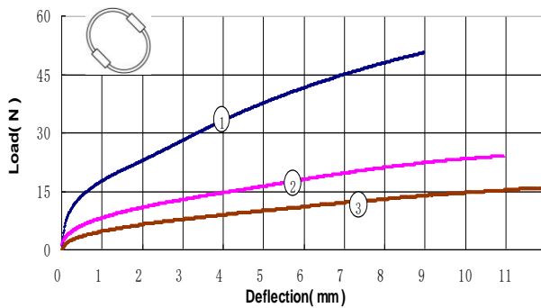
45° Compression
